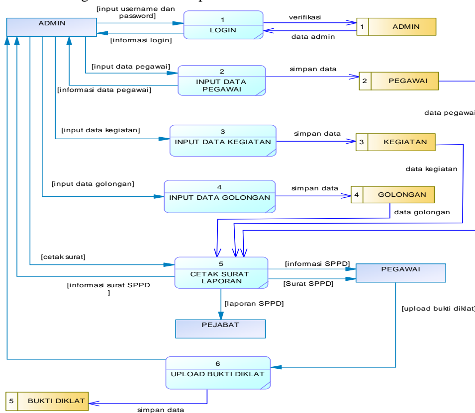
Gambar 2. DFD Level 0
