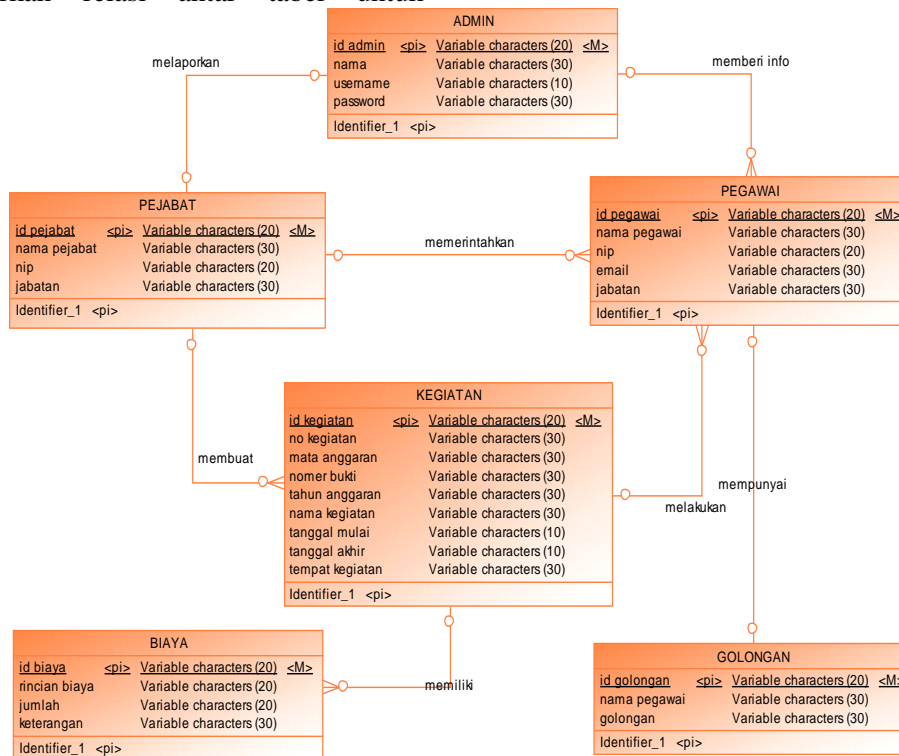
Gambar 3. CDM
