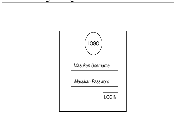
Gambar 4. Interface Login
