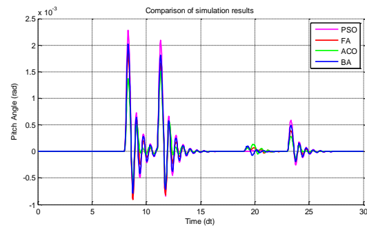
Gambar 7. Hasil Pitch angle masing-masing metode
