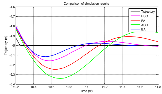
Gambar 6. Hasil overshoot, undershot dan settlingtime masing-masing metode
