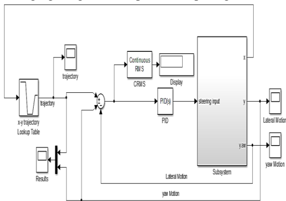
Gambar 4. PID Controller for Vehicle
