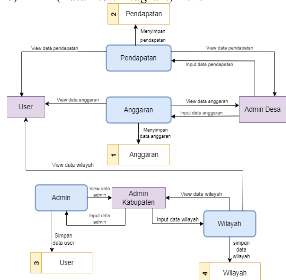
Gambar 5. DFD Level 1
