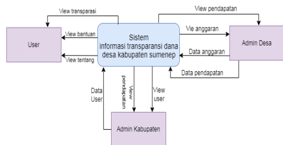
Gambar 4. DFD Level 0
