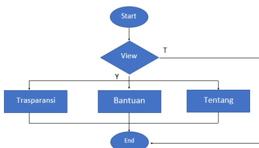
Gambar 3. Flowchart User
