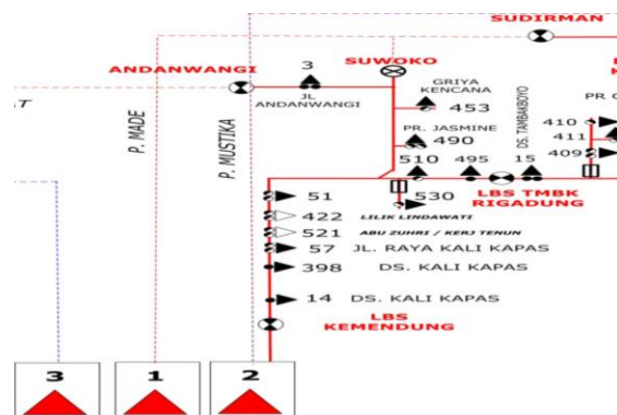
Gambar 2 Single Line Lbs Tambak Rigadung
