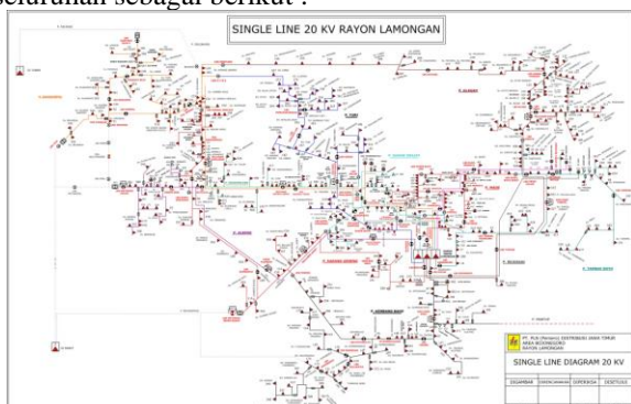
Gambar 1 Single Line Keseluruhan Di PT. PLN (persero) Lamongan
